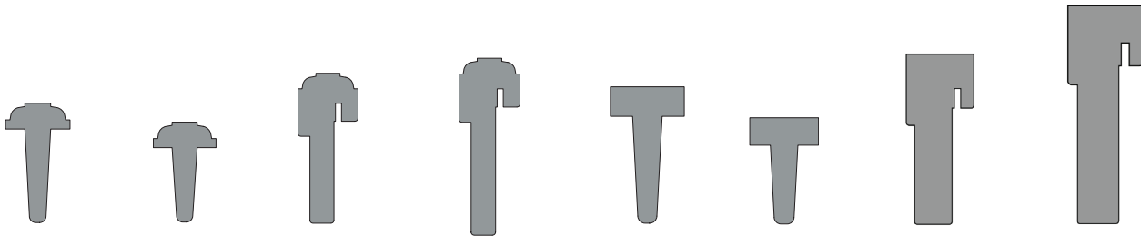
10101 For 1-3/4" Interior Doors 1-1/4" x 2-1/2" 10102 For 1-3/8" Interior Doors 1-1/4" x 2" 10103 For 1-3/4" Exterior Doors 1-1/4" x 3-1/8" 10107 For 2-1/4" Exterior Doors 1-1/4" x 3-5/8" 10104 For 1-3/4" Interior Doors 1-1/4" x 2-1/4" 10105 For 1-3/8" Interior Doors 1-1/4" x 1-3/4" 10106 For 1-3/4" Exterior Doors 1-1/4" x 3-1/8" 10108 For 2-1/4" Exterior Doors 1-1/4" x 3-5/8"
